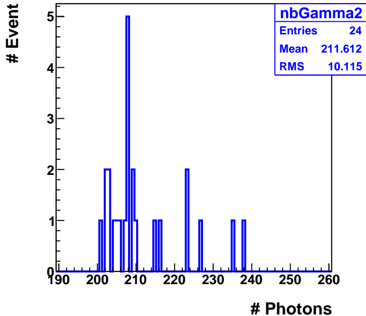
Distribution of Photons in 24 Event
