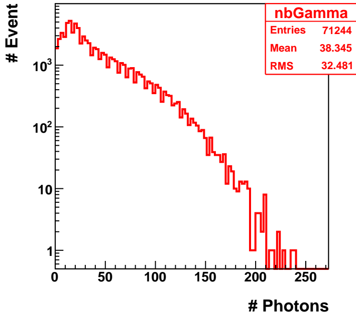
Distribution of Photons in All Event
