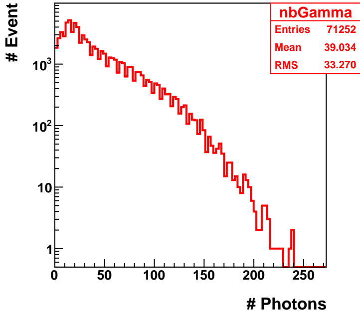
Distribution of Photons in All Event
