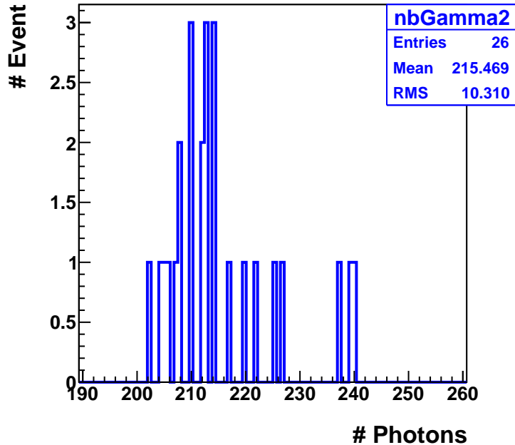
Distribution of Photons in 26 Event
