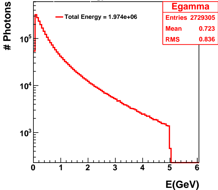
Energy of All Photons
