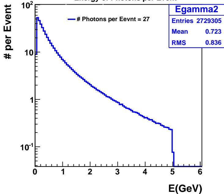
Energy of Photons per Event
