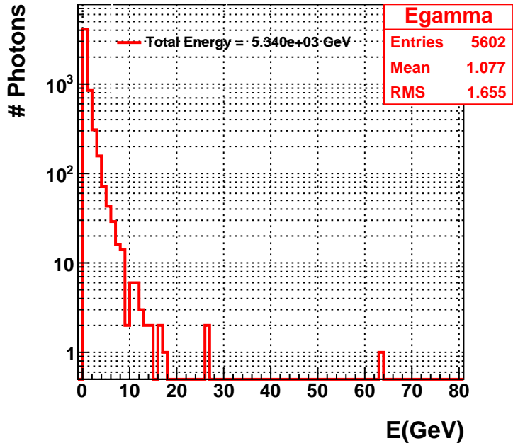
Energy of Photons in 26 Event
