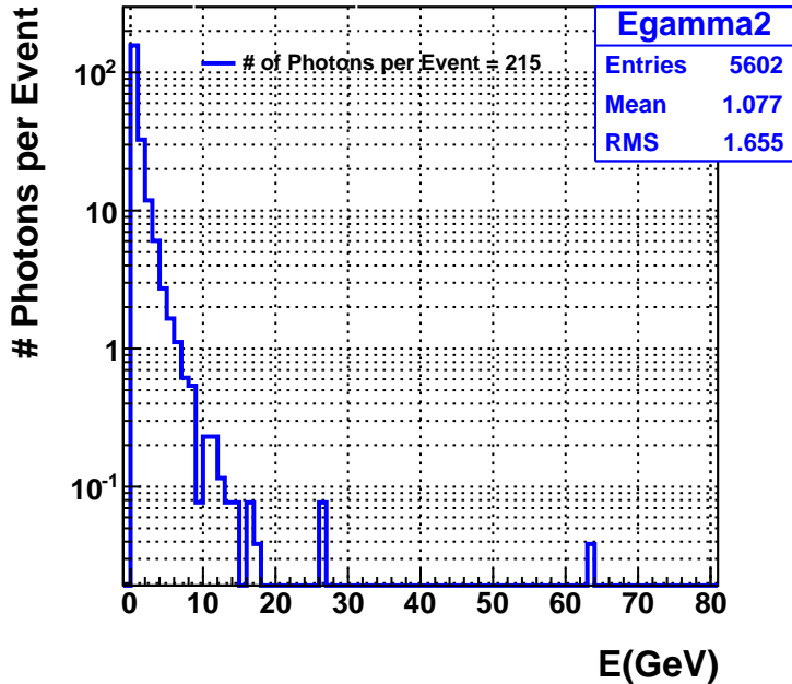
Energy of Photons per 26 Event
